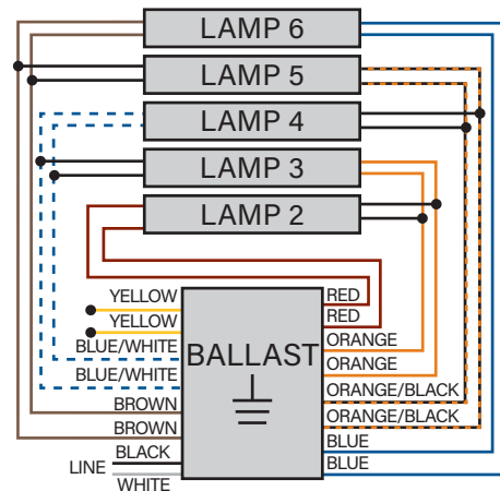
Five Lamp Application, Cap Off Unused Leads Individually, Insulate to 600V
