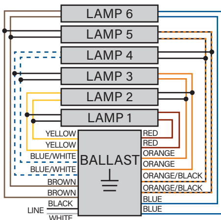
Six Lamp Application
