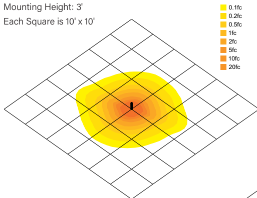
CONE REFLECTOR
