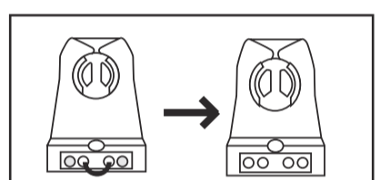
Figure 2.-External shunted Lampholder
