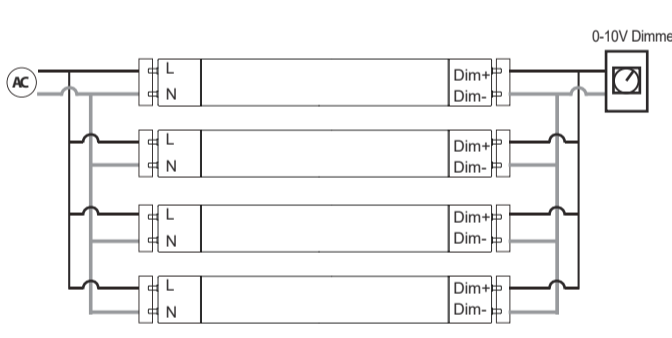
Figure 4. - Multiple lamps wiring
