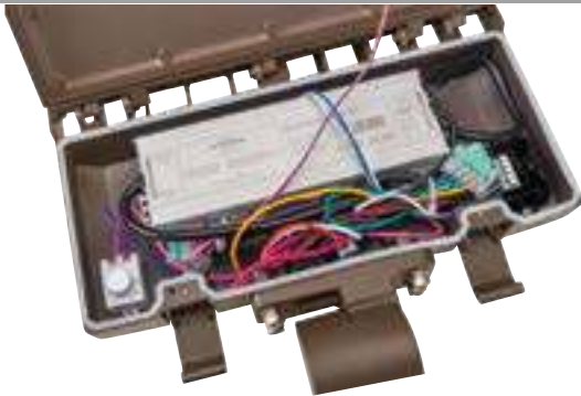
EASILY ACCESSIBLE KEYSTONE DRIVER
