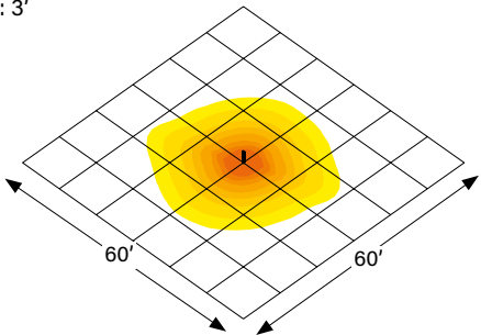
Bollard with Cone Reflector Mounting Height: 3'
