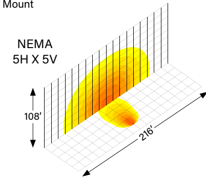
290W High Powered Floodlight with Ground Mount
