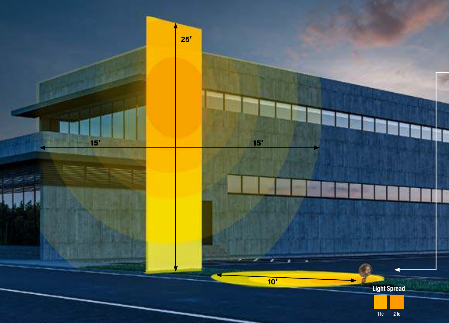
25W Bullet Floodlight: Aimed 45° above horizontal 10' from building 6" above ground; 4x4 optics
